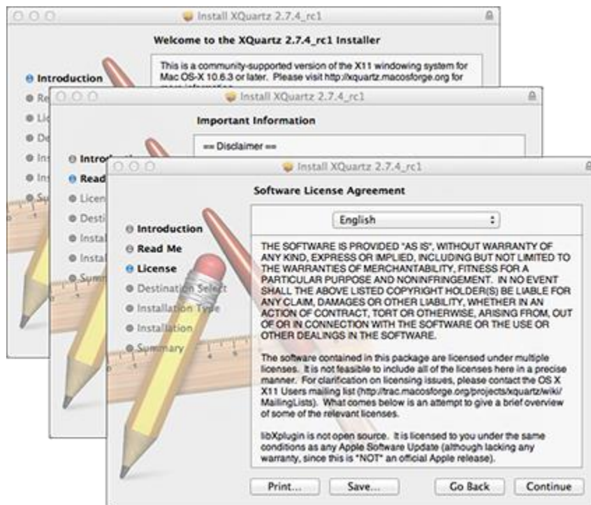
Obr. 5. Instalace Xquartz
