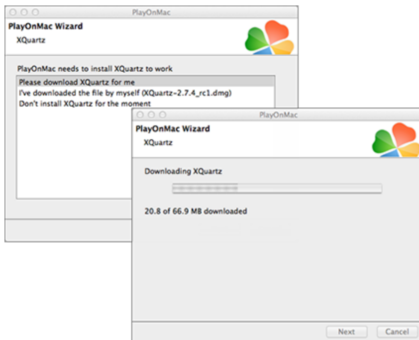
Obr. 4. Instalace Xquartz
